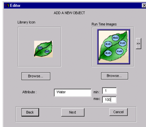
Figure 3. Primitive Object Editor
